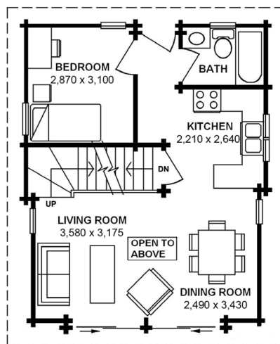
MAIN FLOOR 41.93 m 2 (15.71 坪)
