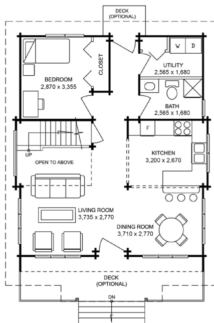
MAIN FLOOR 70.30 m 2 (21.26 坪)
