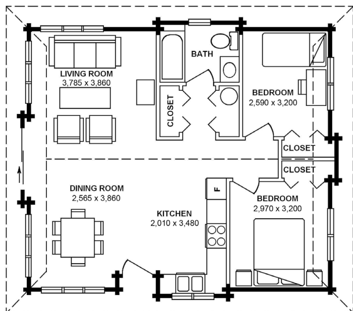
MAIN FLOOR 73.55 m 2 (22.25 坪)
