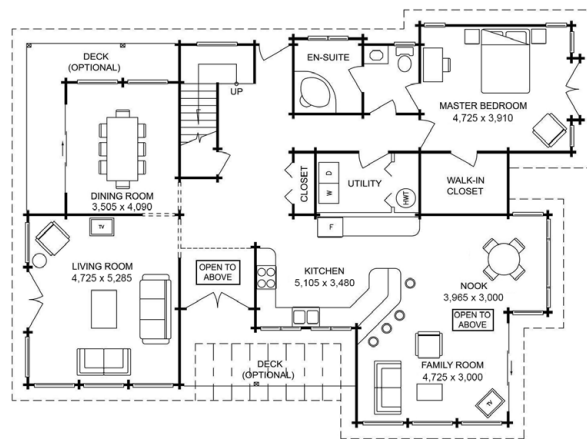
MAIN FLOOR 164.51 m 2 (49.77 坪)
