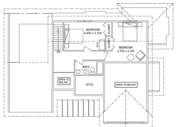
UPPER FLOOR 51.82 m 2 (15.67 坪)
