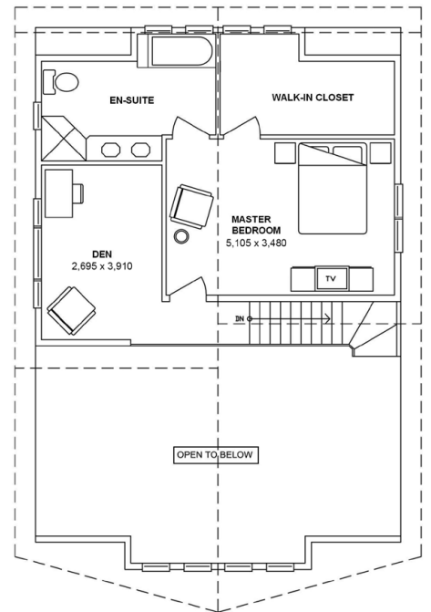
UPPER FLOOR 52.22 m 2 (15.80 坪)
